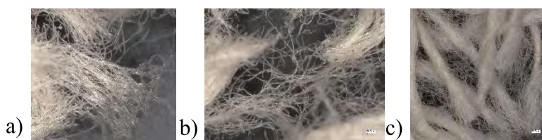
Figure 2: Optical microscopy of deweaved cotton fibers with biopolymer (a), UV-treated biopolymer (b), and water (c).
