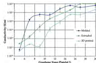
Figure 1. Electrical conductivity of molded, extruded, and 3D printed PLA/PBAT-graphene nanocomposites vs. GNP content. Conductivity increased with GNP loading. Percolation occurred at 7% (molded) and 11% (3D printed); molded samples had the highest values.
