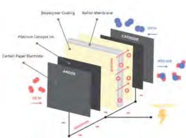
Figure 1: Membrane Electrode Assembly (MEA) using Rhizobium tropici derived biopolymer.
