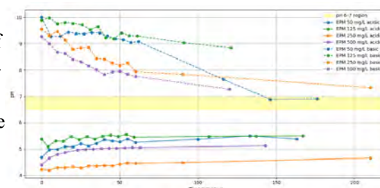
Figure 1: pH vs. Time for Various EPM Concentrations
