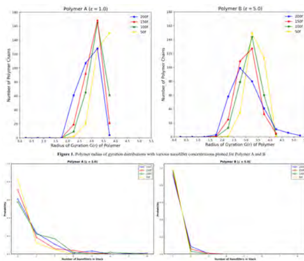
Figure 2. Nanofiller stack size distributions with various nanofiller concentrations plotted for Polymer A and B
