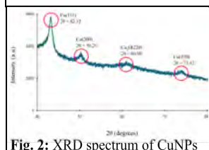
Fig. 2: XRD spectrum of CuNPs
