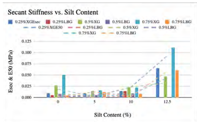
Fig 1. Secant Stiffness vs. Silt %
