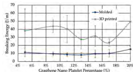
Figure 3. Breaking energy of molded and 3D printed PLA/PBAT-graphene nanocomposites across 4–20% GNP weight from impact testing. 3D printed samples were consistently stronger than molded, and showed no significant increase in brittleness with increasing GNP %.
